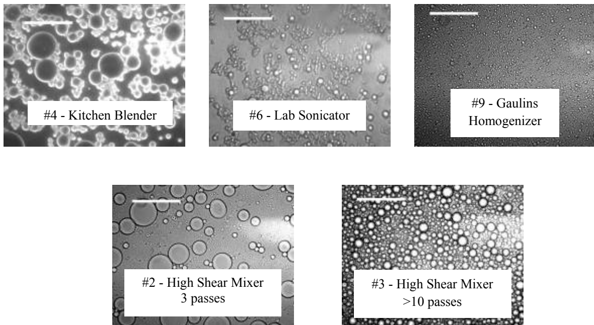
Figure D.4 Emulsion Droplets Produced with Different Surfactants and Mixing Devices (as described in Table D.4, white scale bar is 25 μm)
